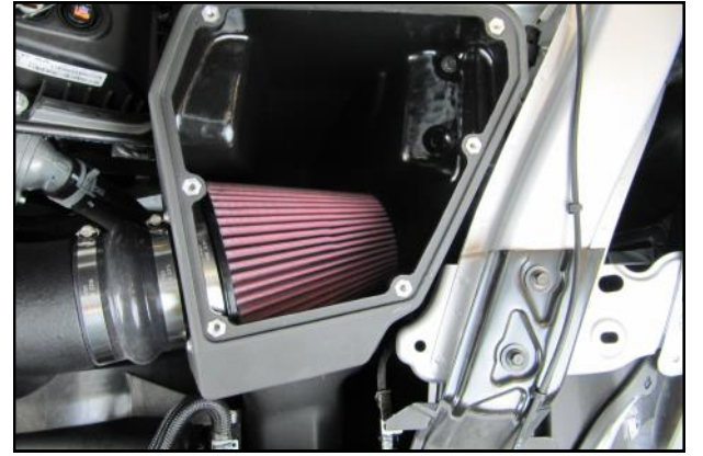
12. Install the Airaid Premium Filter onto the Filter Adapter inside of the Airbox
