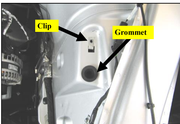
4. Be sure to retain the speed clip in the inner fender, and replace the grommet if it comes out with the air box.
